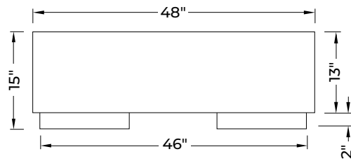
SIDE VIEW - BASE
