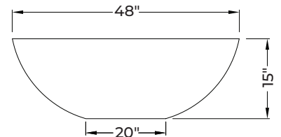
SIDE VIEW - BASE
